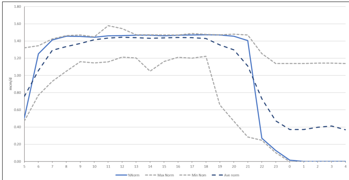
Figure 14 Normalised linepack depletion profile in the South West, based on 25 highest days between 2017 and 2020
