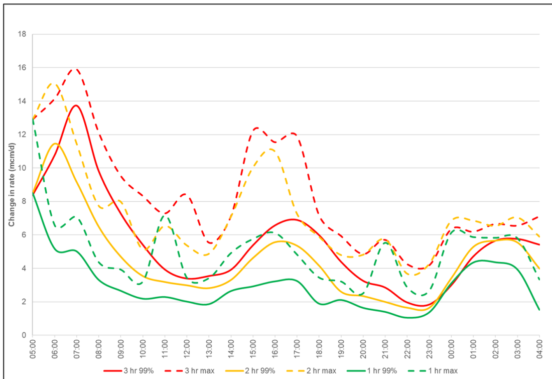
Figure 15 Changes in CCGT demand over time in the South West region between 2017 and 2020.
