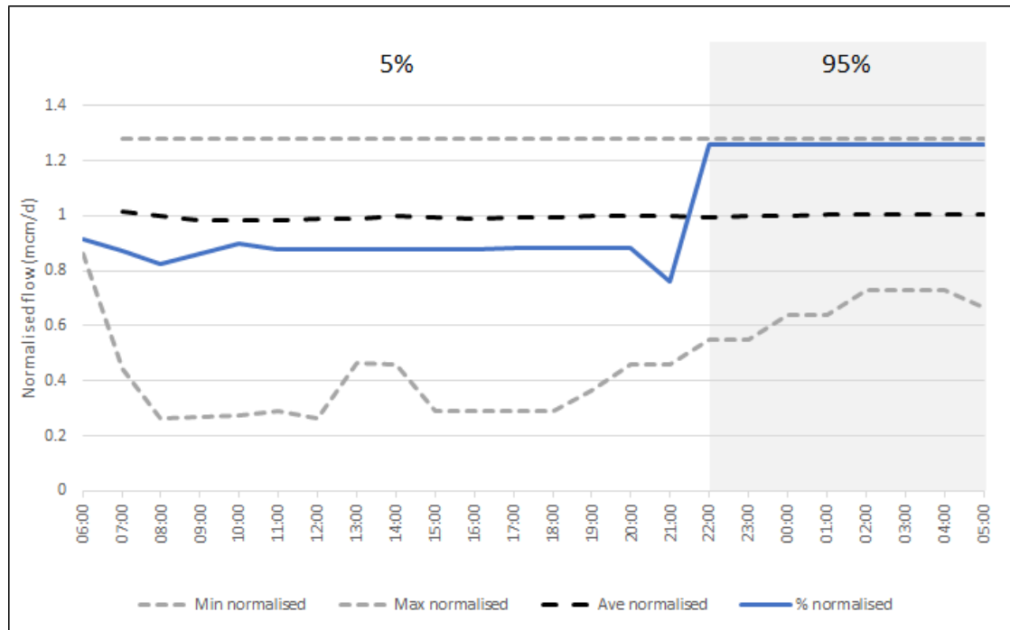
Figure 9 Example of a normalised supply profile for a site between 2017 and 2020, with maximum, minimum and average profiles.
