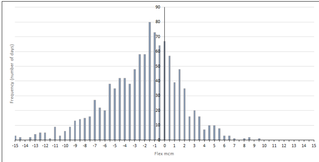
Figure 8 Number of instances of a given total supply driven linepack depletion 2017 to 2020
