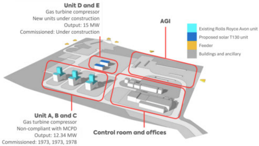
Figure 6: Current setup at [REDACTED]
