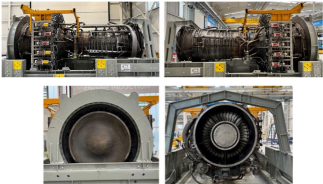
Image 24: Aberdeen LM2500 Gas Generator Overhaul – engine delivered to site and positioned within transport container ahead of planned overhaul activities
