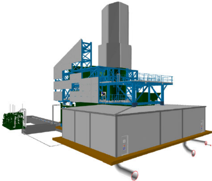
Figure 7: Unit F Acoustic Design
