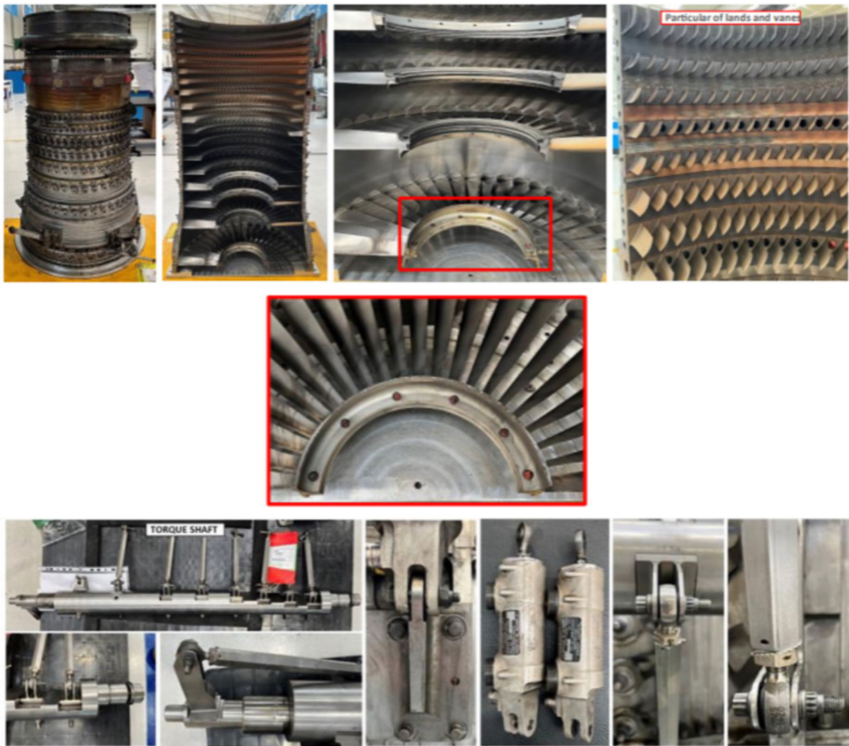
Image 26: [redacted] LM2500 Gas Generator Overhaul – Inspection of the high-pressure compressor stator and variable stator vane (VSV) system, identifying wear, fouling and component condition to inform refurbishment and ensure optimal performance on return to service
