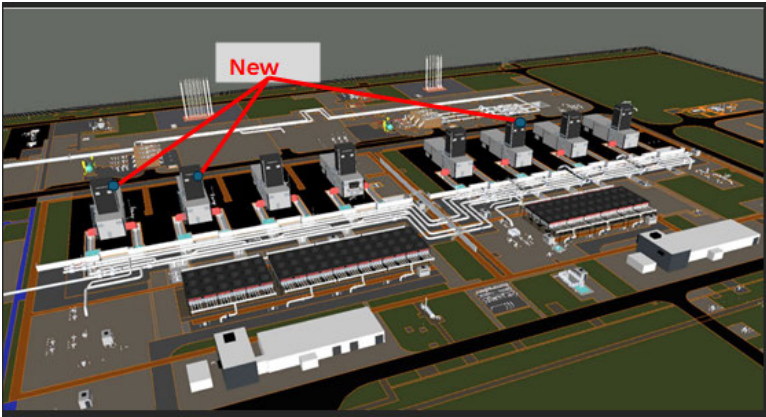
Image 4: Plant 1 and Plant 2 layout identifying units to be replaced
