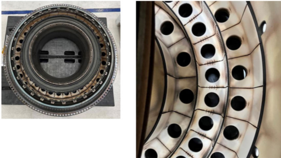
Image 32: [REDACTED] LM2500 Gas Generator Overhaul - Inspection of the combustor assembly, assessing liner condition, thermal wear and combustion integrity to support refurbishment and reliable operation on return to service
