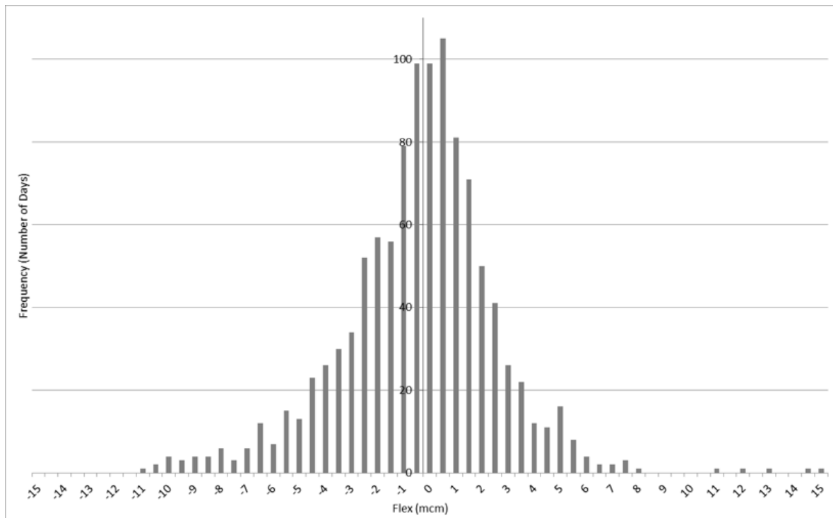
Figure 8 Number of instances of a given total supply driven linepack depletion 2020 to 2023
