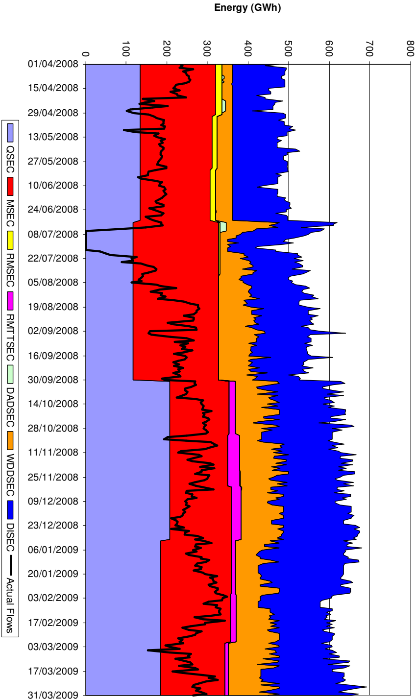
Capacity Sold vs Actual Flows - Teesside 01 April 2008 to 31 March 2009
